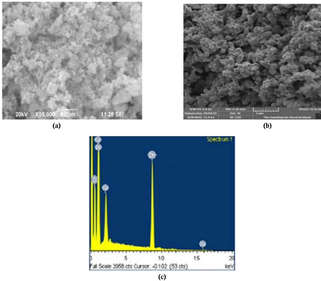
Figure 4. (a) SEM image of CZ5. (b) SEM image of CZ8. (c) EDAX image of CZ5.
