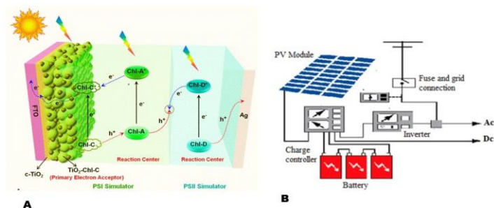
Figure 2. (a) Triple-layer chlorophyll-based bio-solar modules [17]; (b) Schematic diagram of BIPV [17].
